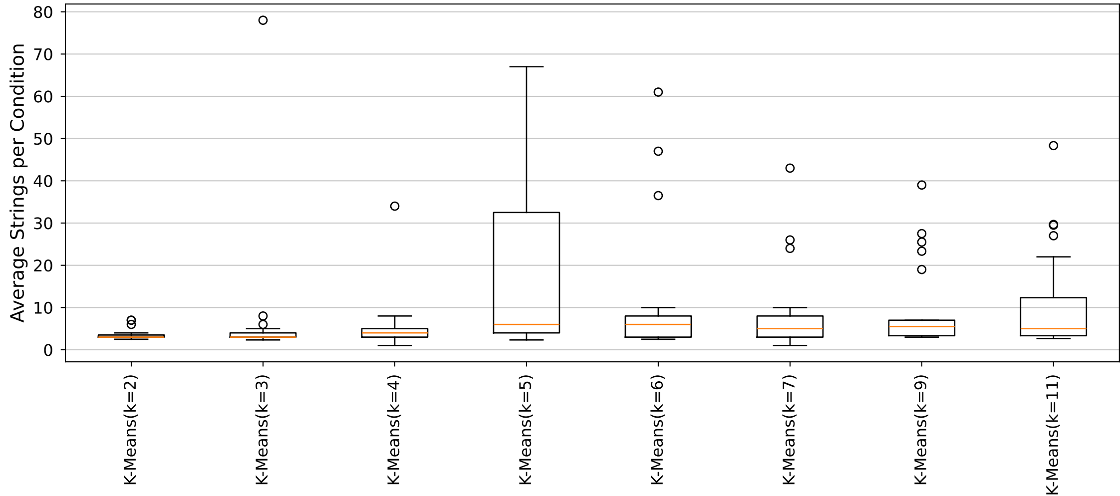
YARA Rules Average Strings per Condition Distribution (Cluster9_Size11 dataset)
